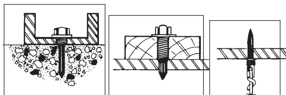
Figure 40-4: Types of Studs
